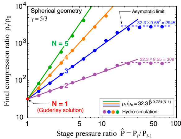
Figure 1. Final compression \rho_r/\rho_0 versus stage pressure ratio \hat{P} for N = 1 – 5 stacked shocks. \rho_r is the reflected-shock crest density immediately after on-axis coalescence and is subsequently advected outward with the diverging shock. Dashed lines indicate the asymptotic limits.
